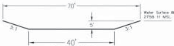
APPROXIMATE CROSS SECTION OF DREDGE CHANNEL
